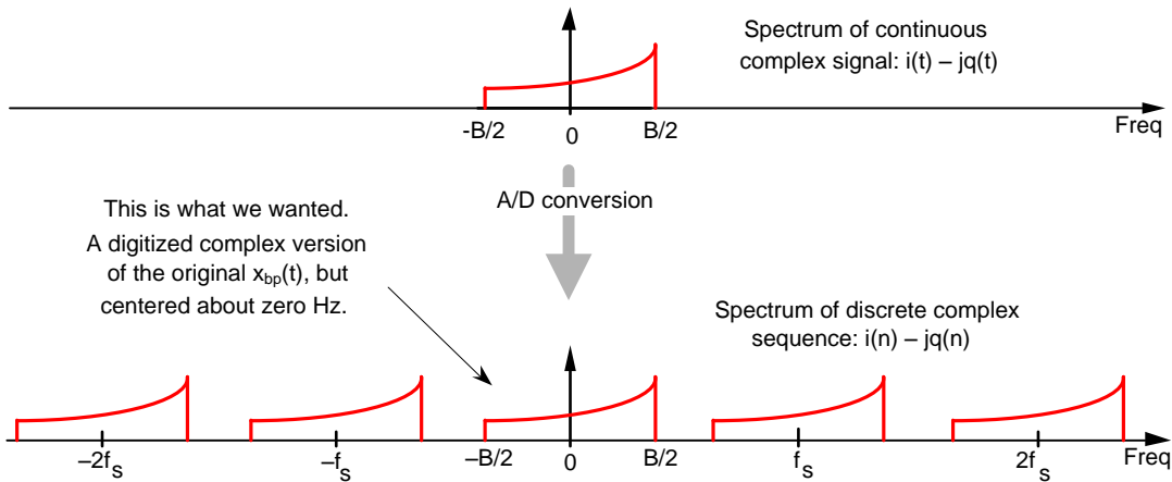
Figure 18. The continuous complex signal i(t) - jq(t) is digitized to obtain the discrete i(n) - jq(n) .
